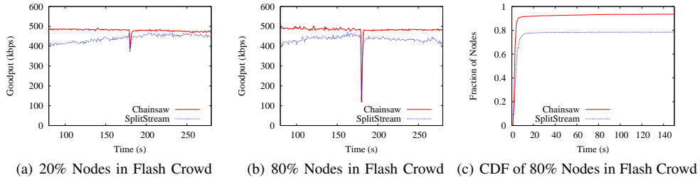
Fig. 7. Performance for different percentages of flash crowds using a configuration of 280 nodes with bandwidth greater than 1 Mbps
