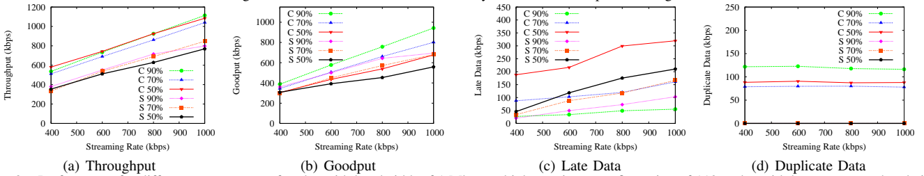
Fig. 3. Performance for different percentages of nodes with bandwidth of 1 Mbps or higher, using a configuration of 112 nodes with heterogeneous bandwidth capabilities. In the figure, “C” denotes Chainsaw and “S” denotes SplitStream
