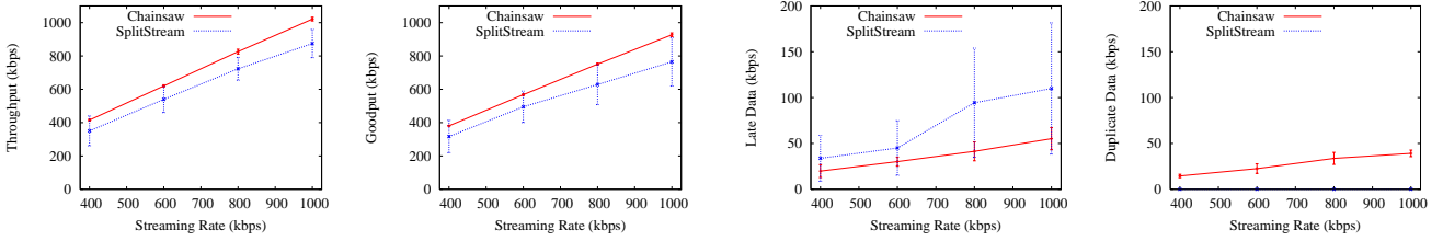
Fig. 1. Performance for different streaming rates using a configuration of 280 nodes with bandwidth greater than 1 Mbps
