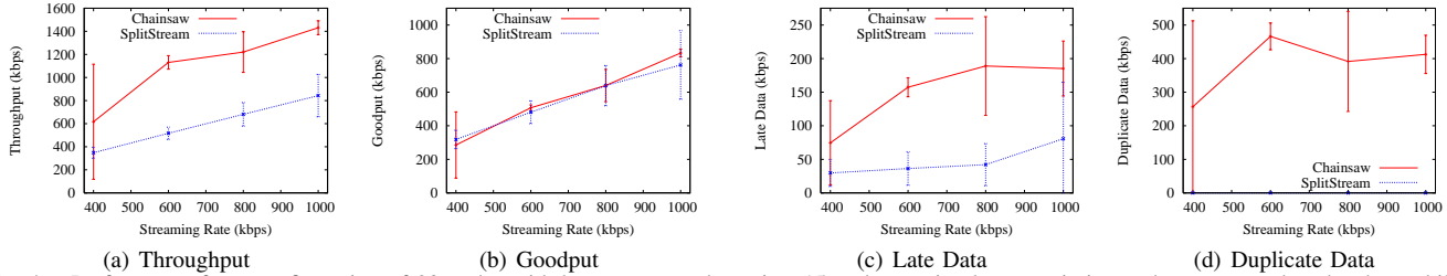
Fig. 4. Performance for a configuration of 20 nodes with heterogeneous latencies: 15 nodes are in close proximity to the source and each other, while the remaining 5 have longer latencies to these 15 nodes and the source
