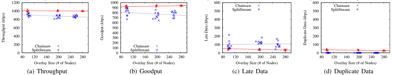
Fig. 2. Performance for different overlay sizes for a 1 Mbps streaming rate
